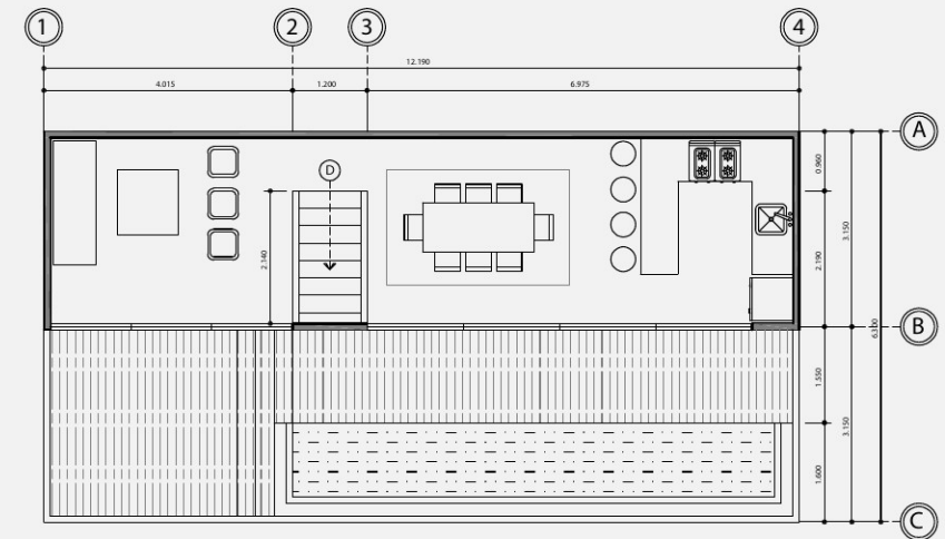
2nd Floor Med Suite - 77 m 2 - 829 ft 2 Social area / Private Infinity Pool + Deck
