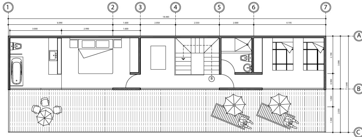
2nd Floor The Lake House - 104.5 m 2 - 1125 ft 2 2 Bedrooms / 2 Bathroom / Deck
